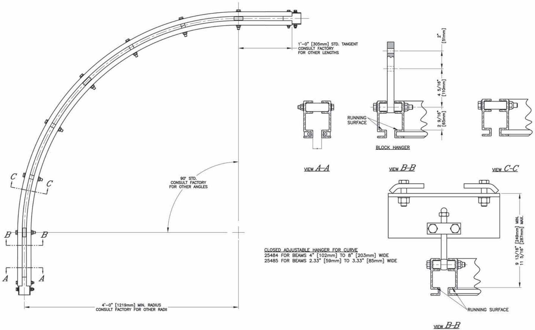
ETA-4 CURVED RAIL
