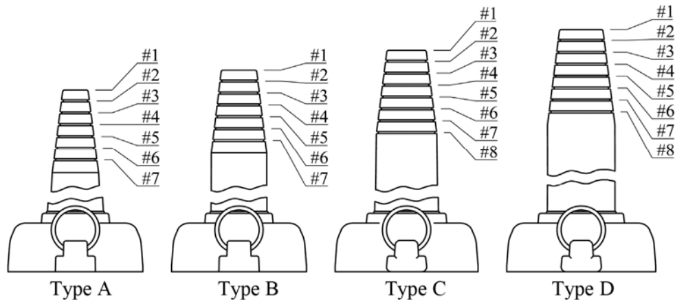
Figure 6: Cable Armor Types and Cutting Points
